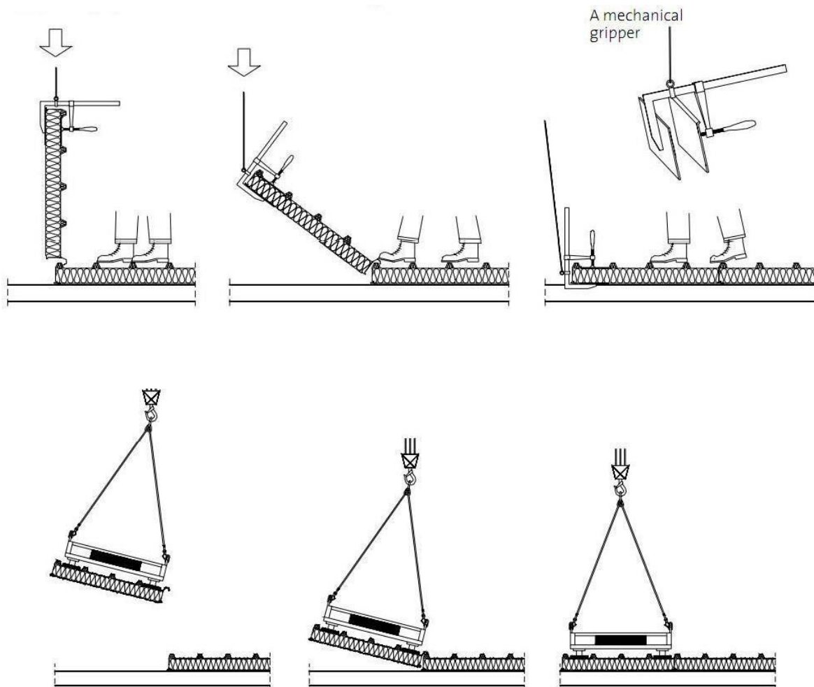
Fig. 8. Assembly of panels using mechanical grippers.
