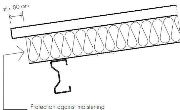
Fig. 6. Dripping edge.
