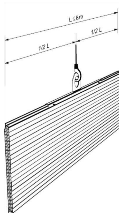
Fig. 17. Clamp application L \leq 6m .
