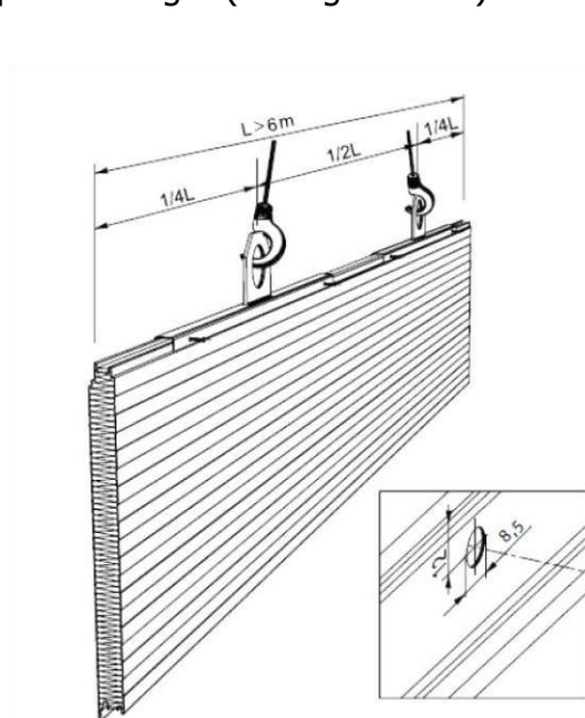
Fig. 16. Clamp application L > 6m .
