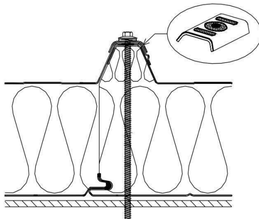
Fig. 3. Correct fixation of the self-drilling fasteners
