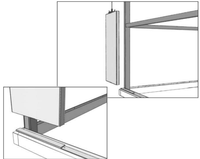
Fig. 14. Insulation wool in the bottom edge.
