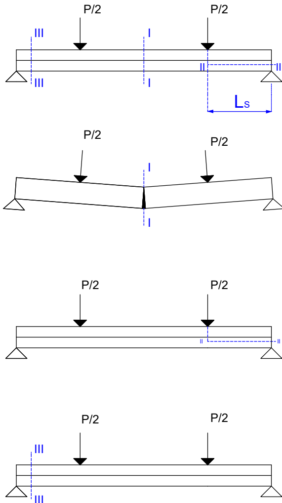
Figure 4: Failure modes of composite slabs.
