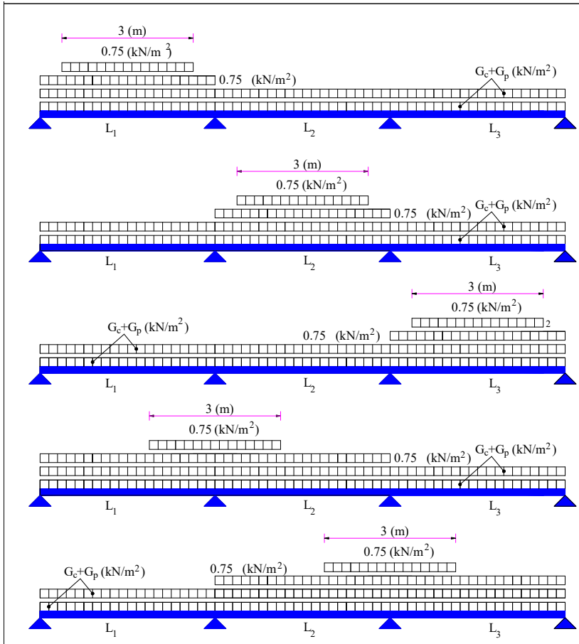
Figure 10: Load combinations for “progressive” casting.
