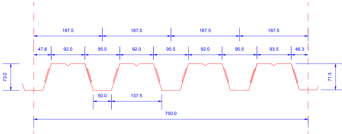
Figure 3: Geometry of the SYMDECK73 trapezoidal steel sheeting
