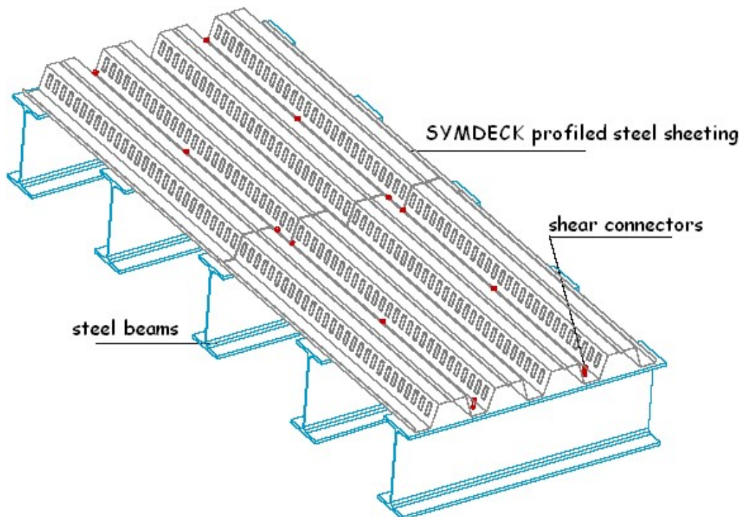
Figure 1: Typical configuration of a composite slab.
