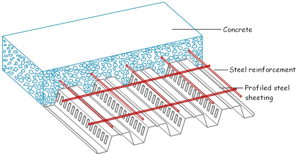
Figure 2: Typical composite slab
