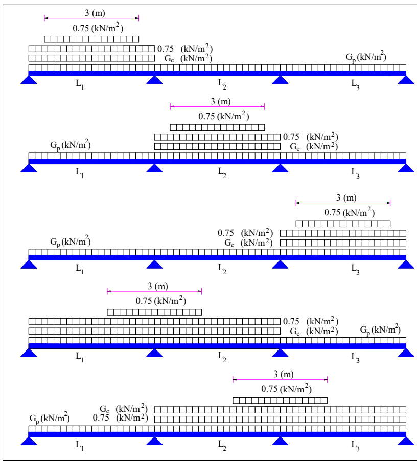
Figure 9: Load combinations for “span-by-span” casting.
